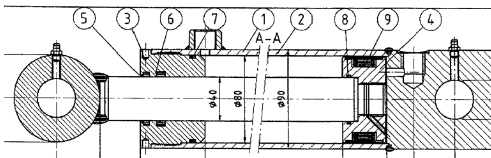
Vérin 80/40-350 (91805)
