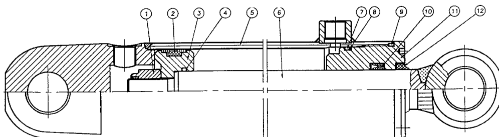
Cylinder 70/30-205
