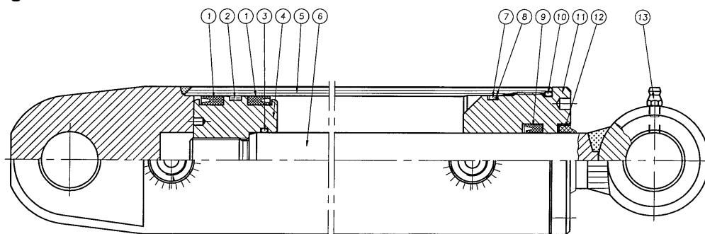
Cylinder 70/30-205
