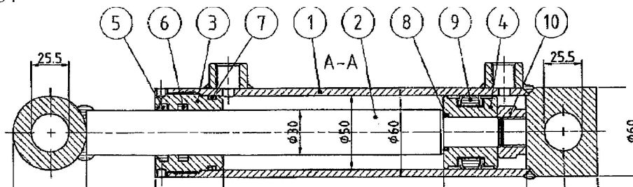
Cylinder 50/30-150
