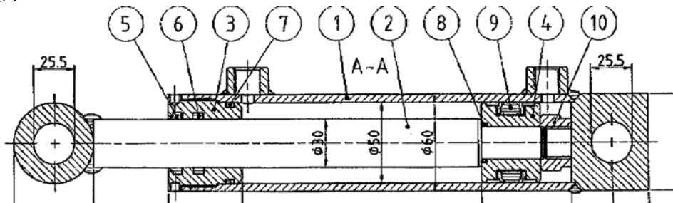
Cylinder 50/30-150
