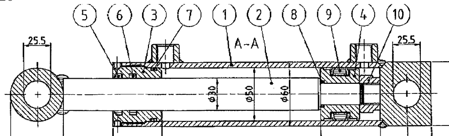
Cylinder 50/30-150
